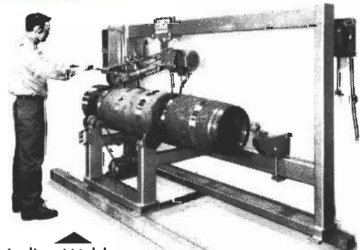
Grinding Weld
